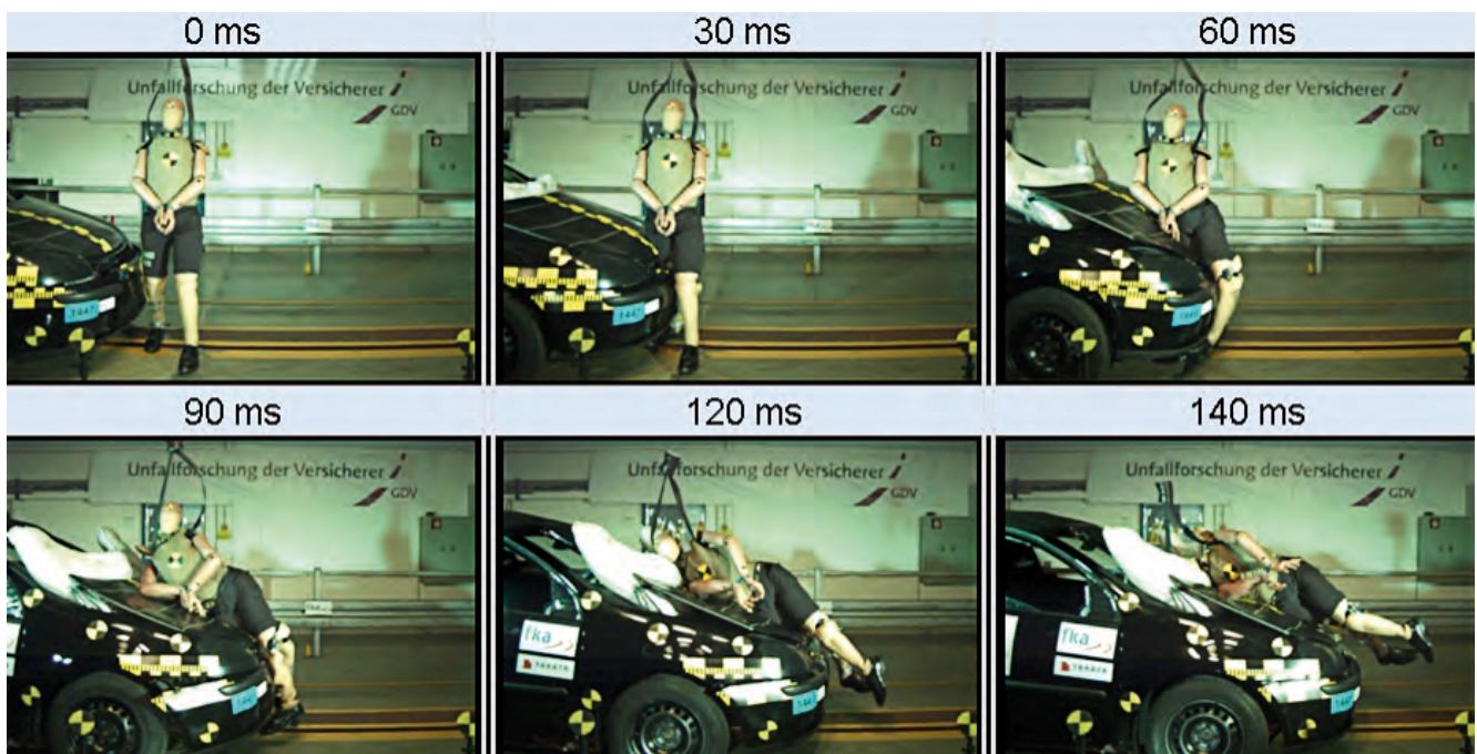
Figure 8: System test (with systems applied) at a vehicle speed of 40 kph
